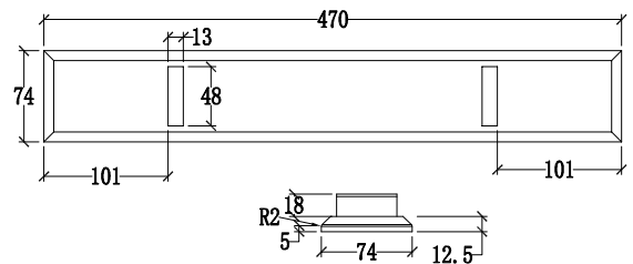
COVER PLATE
